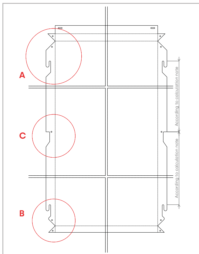
UNFOLDED CASSETTE
