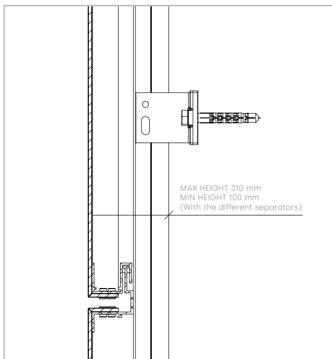
VERTICAL SECTION
